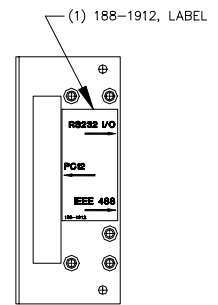
DETAIL "C" REAR BRACKET, 128-1810
