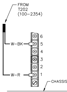
DETAIL "B" BARRIER TERMINAL STRIP PART OF POWER TRANSFORMER (T201)
